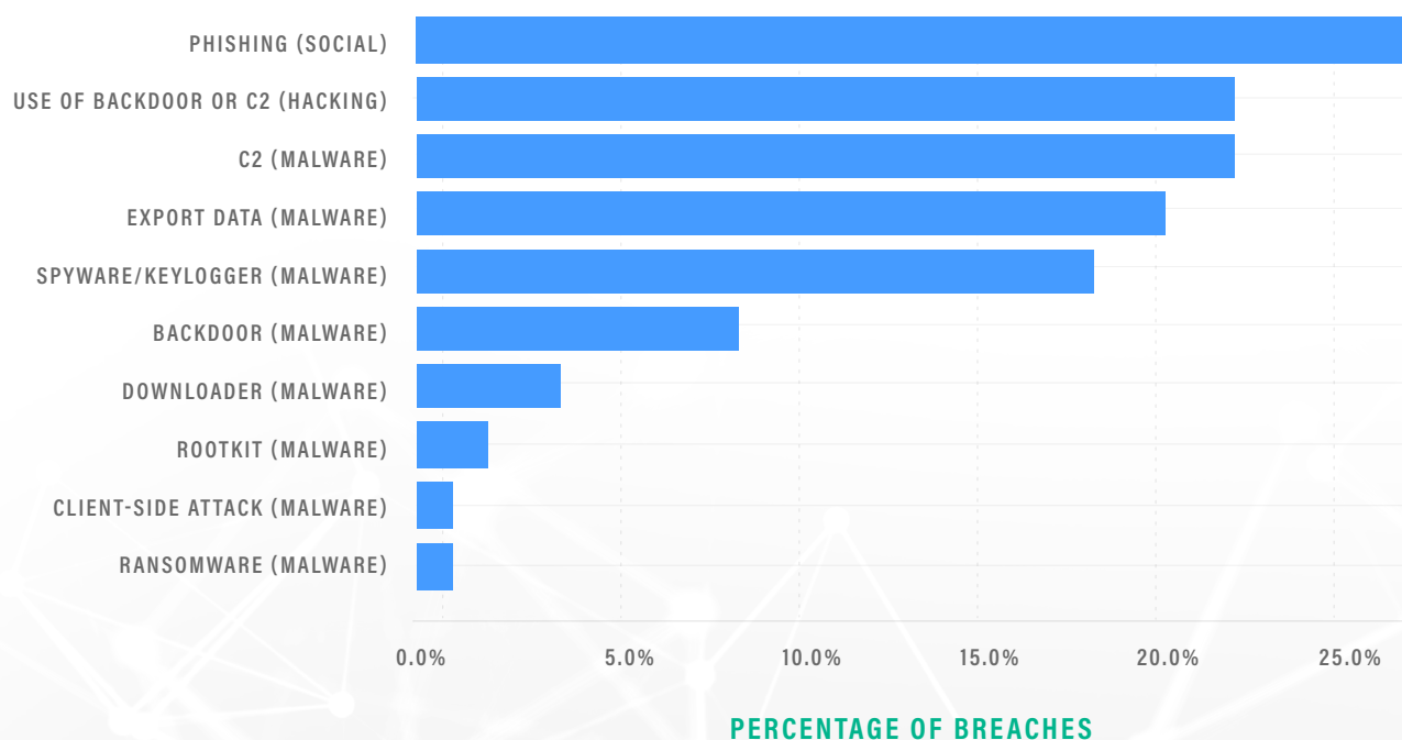
Figure AA: Frequency of VERIS threat actions (and category) in Verizon DBIR Data 2012–2017
